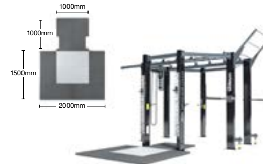
LIFTPLAT5 Integrated Lift Zone - Single Bolted Leg
