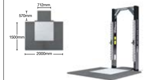
LIFTPLAT8 Integrated Lift Zone - MONO Bolted Leg
