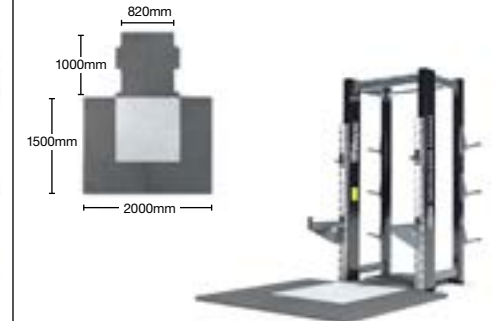
LIFTPLAT6 Integrated Lift Zone - Double Bolted Leg
